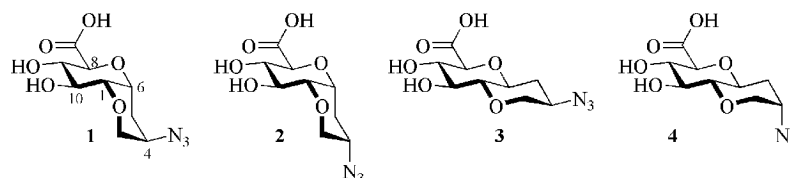
Figure 1. Four isomeric pyranopyran sugar amino acids.
