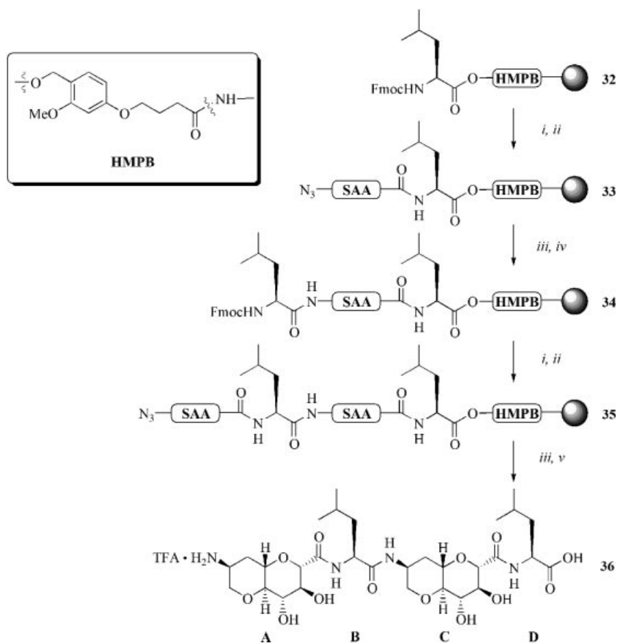
Scheme 3. Reagents and conditions: i ) piperidine/NMP, 1:4 v/v. ii ) 4 , PyBOP, HOBT, DIPEA, NMP. iii ) (a) Me 3 P, dioxane, (b) water, dioxane iv ) FmocLeuOH, PyBOP, HOBT, DIPEA, NMP. v ) TFA: CH 2 Cl 2 1:99 v/v, 36 24% (based on 32 ).
