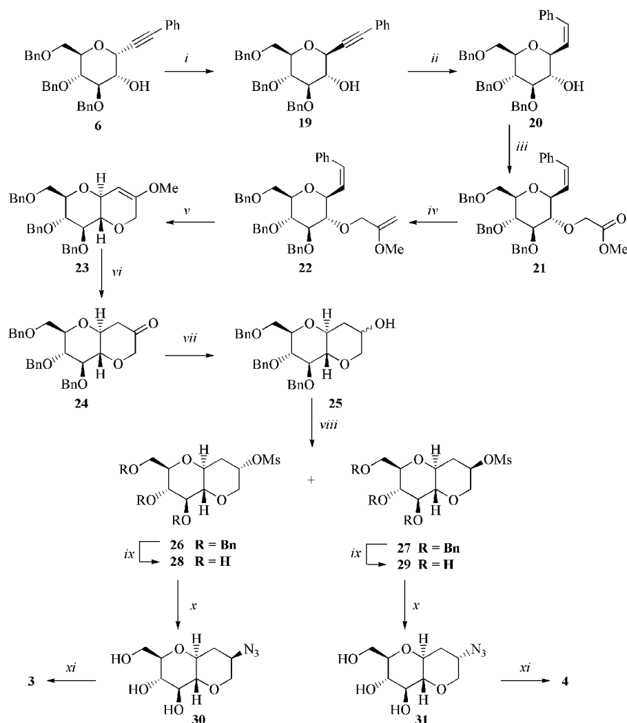
Scheme 2. Reagents and conditions: i ) (a) \text{Co}_2(\text{CO})_8 , \text{CH}_2\text{Cl}_2 , (b) \text{TfOH} , \text{CH}_2\text{Cl}_2 , (c) \text{I}_2 , \text{THF} , [6] ii ) \text{H}_2 , Lindlar's catalyst, \text{EtOAc} , [6] iii ) methyl bromoacetate, TBAI, \text{NaH} , \text{DMF} , 87%, iv ) \text{Cp}_2\text{TiMe}_2 , \text{THF} , 60 °C, 72%, v ) dichlorido(1,3-dimesityl-2-imidazolidinylidene)(phenylmethylene)(tricyclophosphane)ruthenium, \text{CH}_2\text{Cl}_2 , reflux, 86%, vi ) \text{TFA} , water, \text{CH}_2\text{Cl}_2 , 90%, vii ) \text{L-selectride} , \text{THF} , -78 °C to room temp., viii ) \text{MsCl} , \text{Et}_3\text{N} , \text{CH}_2\text{Cl}_2 , 0 °C, 26 36%, 27 43%, two steps, ix ) \text{H}_2 , \text{Pd/C} , \text{EtOH} , 28 quant, 29 95%, x ) \text{NaN}_3 , \text{DMF} , 70 °C, 30 70%, 31 74%, xi ) \text{TEMPO} , \text{NaOCl} , \text{NaHCO}_3 , \text{MeCN} , 0 °C, 4 49%, 3 72%.
